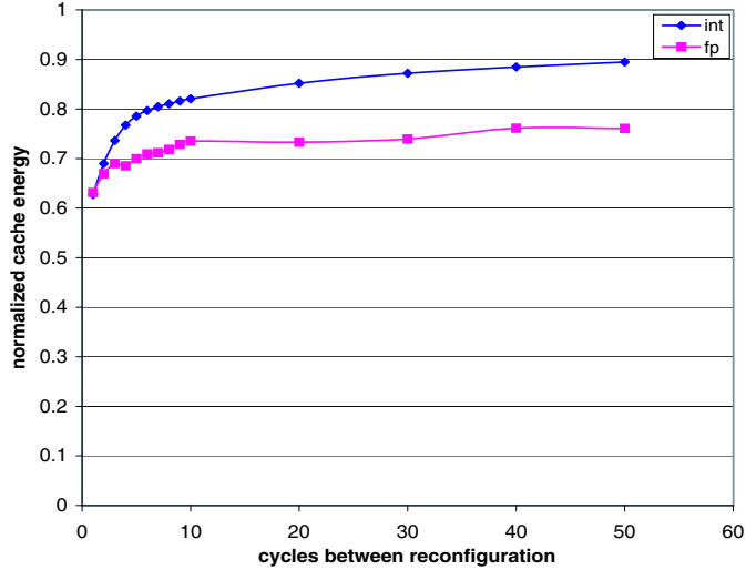
Figure 8: Effect on data cache energy when reconfiguring at different intervals.
