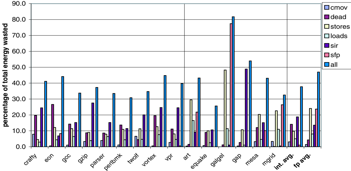
Figure 2: Processor energy waste due to unnecessary instructions and their producers.
