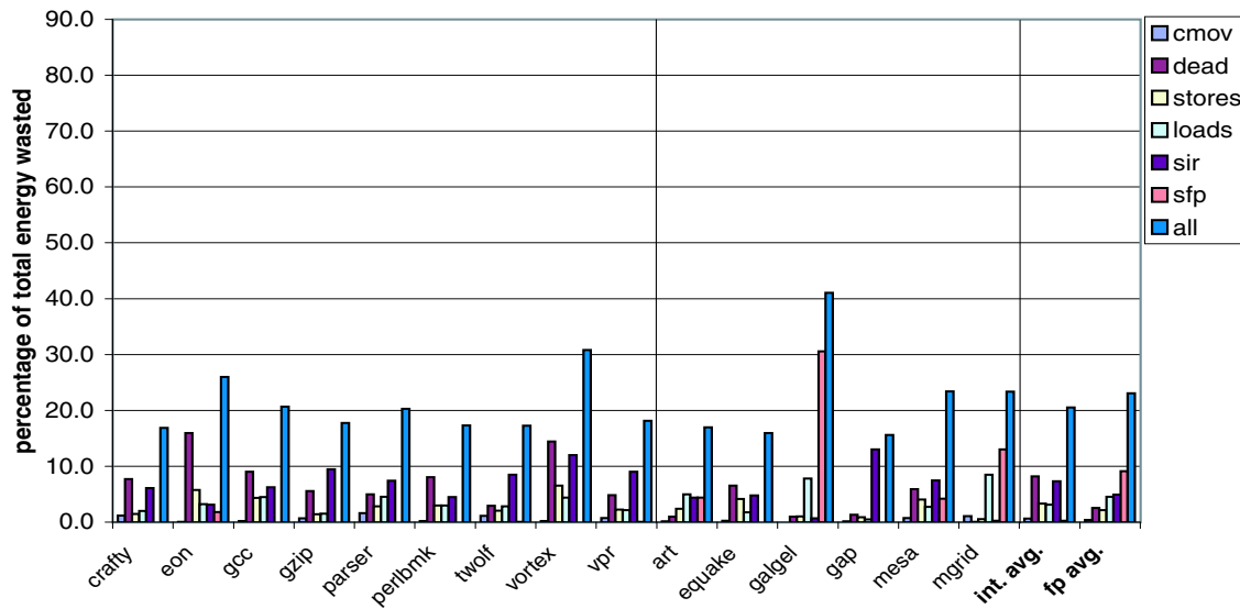
Figure 1: Processor energy waste due to unnecessary instructions.
