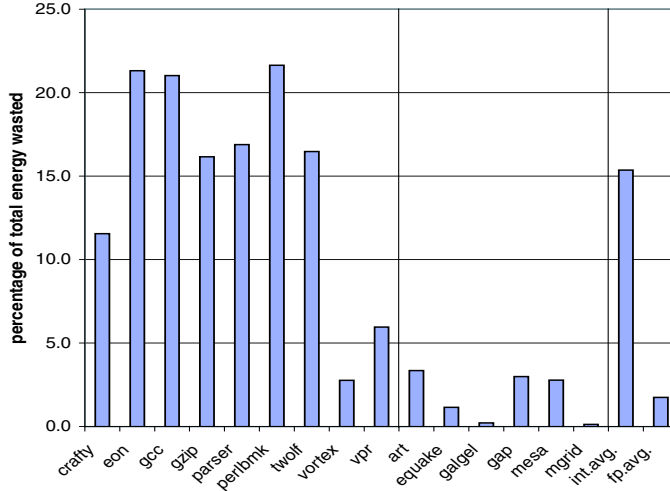
Figure 4: Percentage of total energy that is wasted due to misspeculated instructions.
