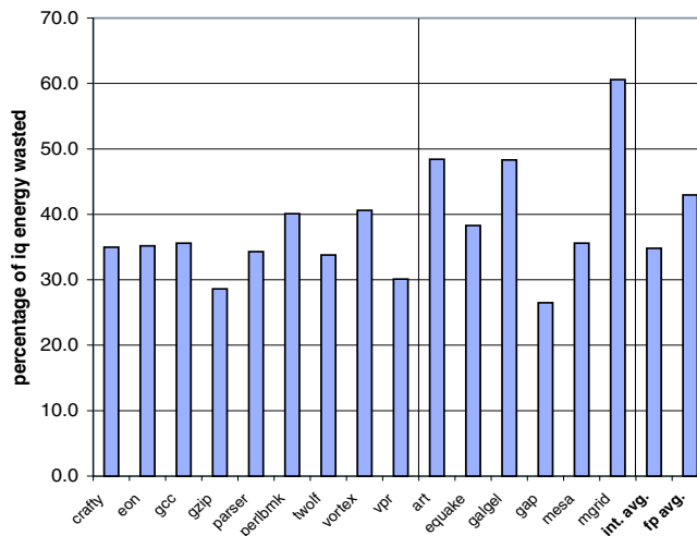
Figure 9: Potential for energy savings available for optimally sized instruction queues.
