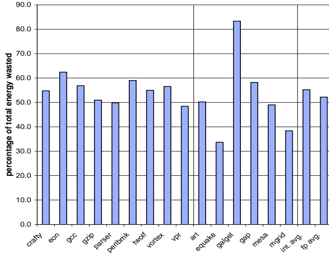
Figure 10: Percentage of total energy that is wasted due to all three sources: program waste, speculation waste, and architectural waste.
